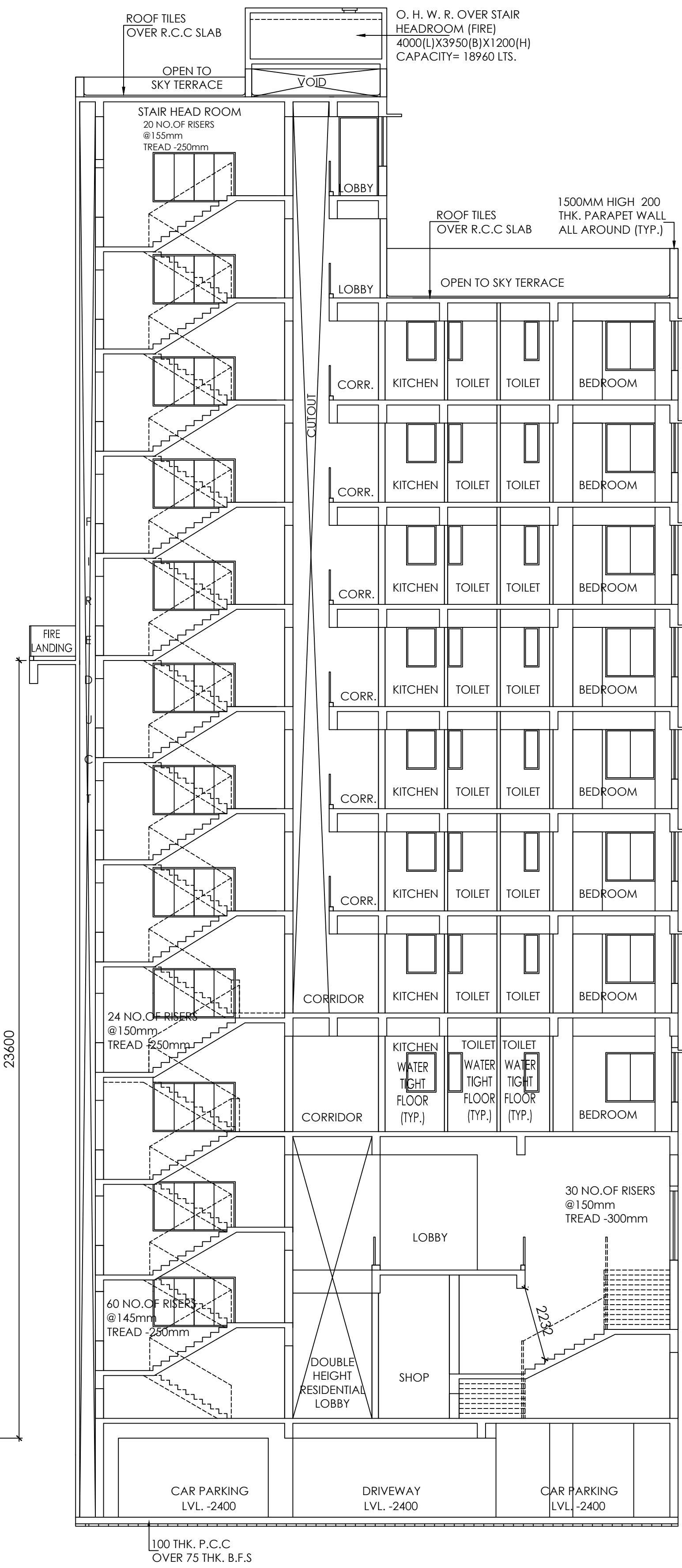
SECTION C-C SCALE - 1:150
